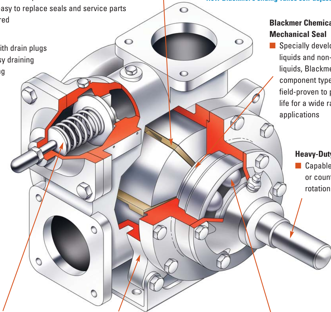
How Blackmer's sliding vanes self-adjust for wear
